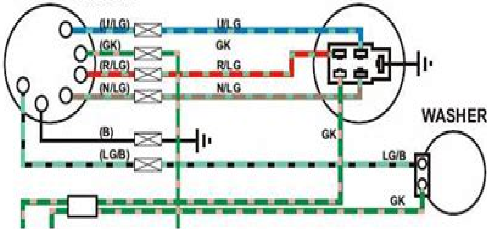
† WIPER/WASHER SWITCH
