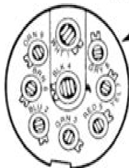
PLUG INTERIOR
