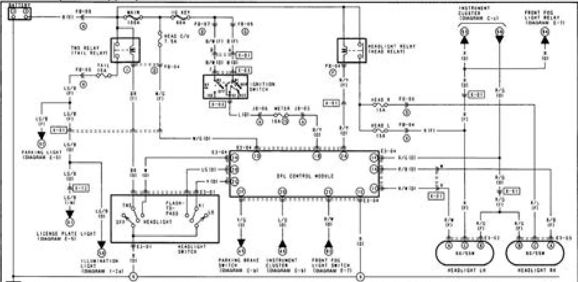
E3-01 HEADLIGHT SWITCH (S)
