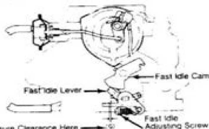
Fig. 132 Adjusting Fast Idle (or throttle) Spring Angle (Courtesy of Mazda Motor Corp.)
