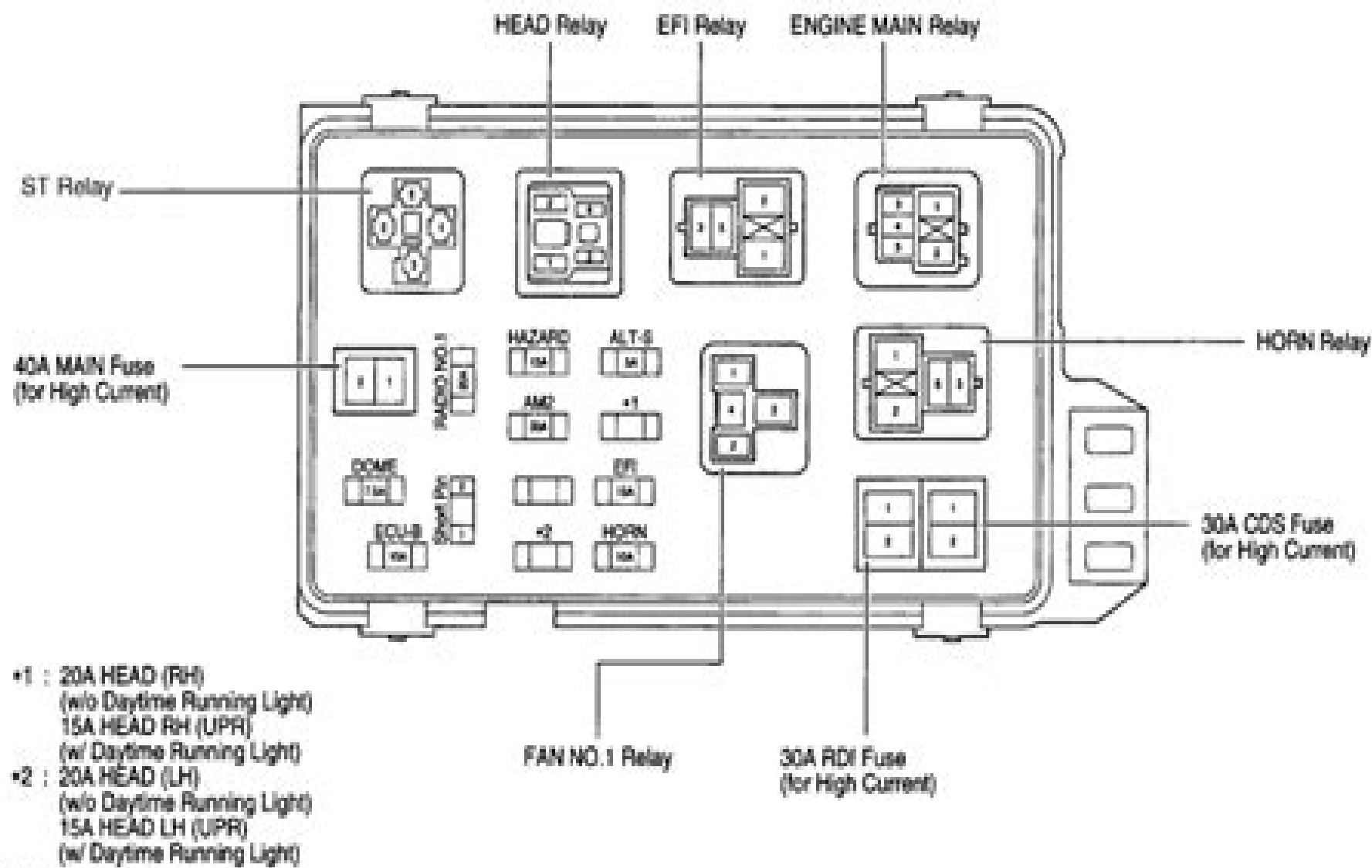
Fig 9: Identifying Engine Room J/B No. 2 Components
