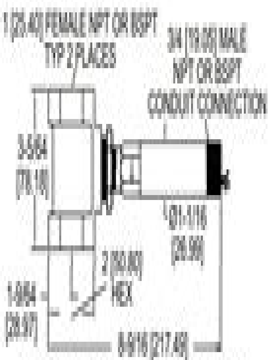
Model L6 with external float chamber
