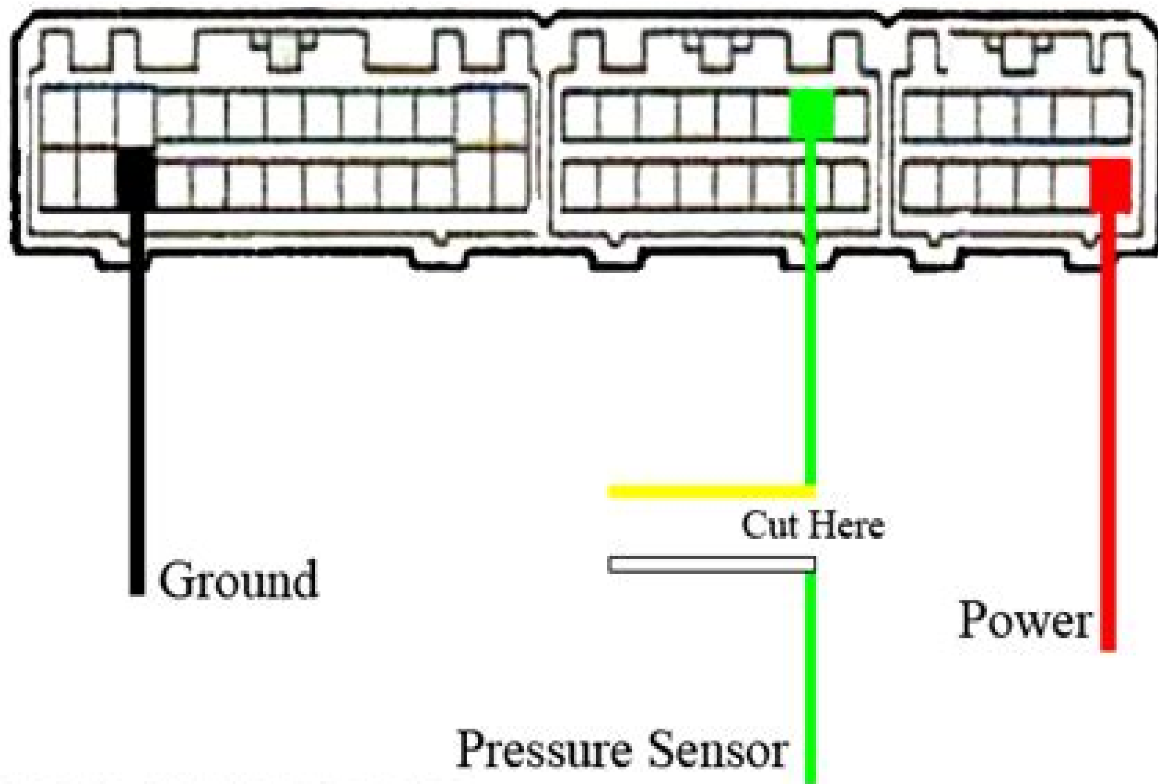
EP91 HKS FCD Wiring Diagram
