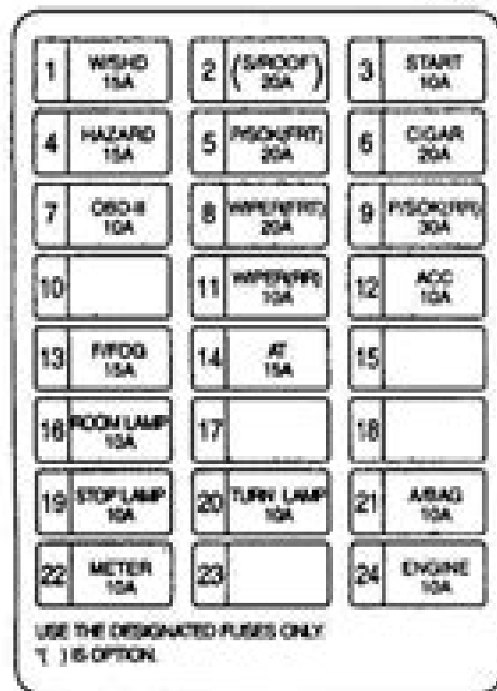
Fig. 2: Locating & Identifying Components On Passenger Compartment Fuse Box Courtesy of KIA MOTORS AMERICA, INC.
