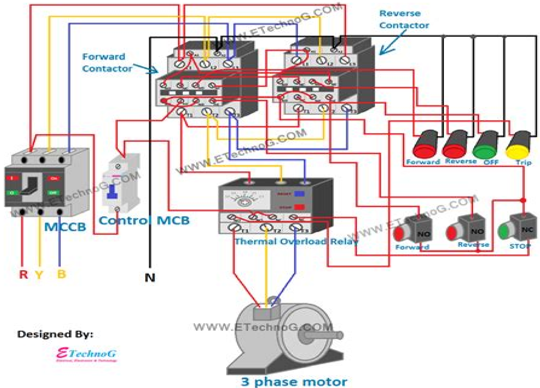
Motor Control Circuit Forward Reverse | Wiring and Connection
