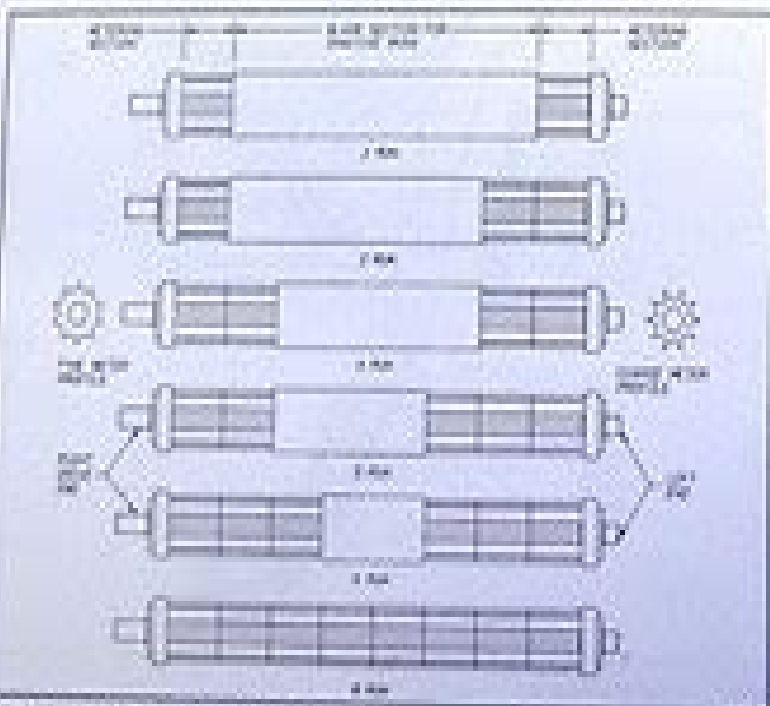
Figure 4.1.2b Meter Rollers for the Meter Line
