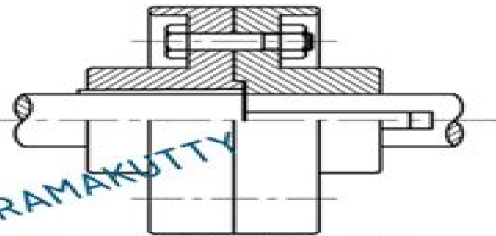
Top Half Sectional Front View
