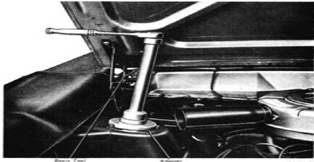
FIG. 9—Spring Compressor Tool Installed—Upper View—Typical
