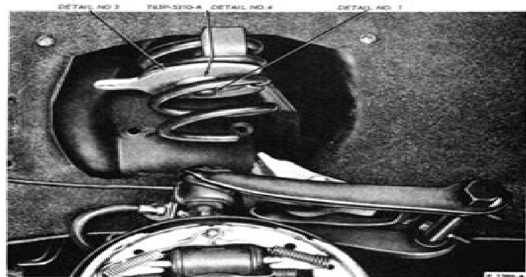
FIG. 10—Compressing Spring—Lower View —Comet, Falcon, and Fairlane
