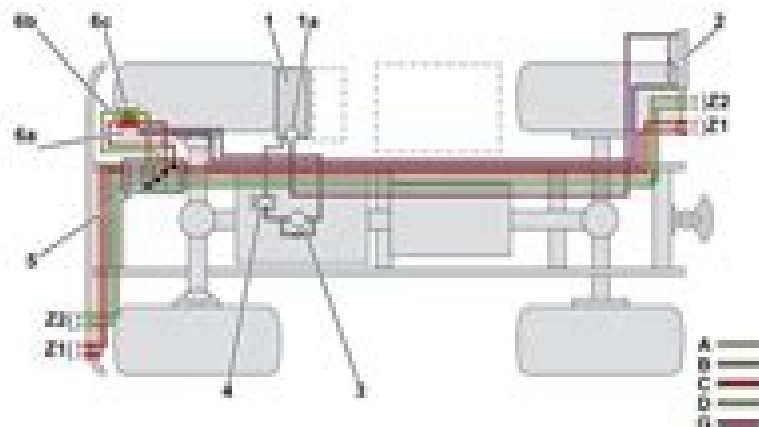
Hydraulic diagram of work hydraulics, front and rear hydraulic system
