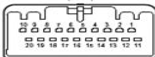
External Device Connector(20P)
