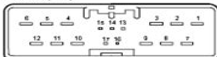
Main Connector(17P)
