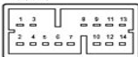
GA-NET Connector(14P)
