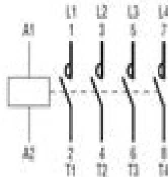
415 VAC 3phase Magnetic Contactor with 230 VAC coil
