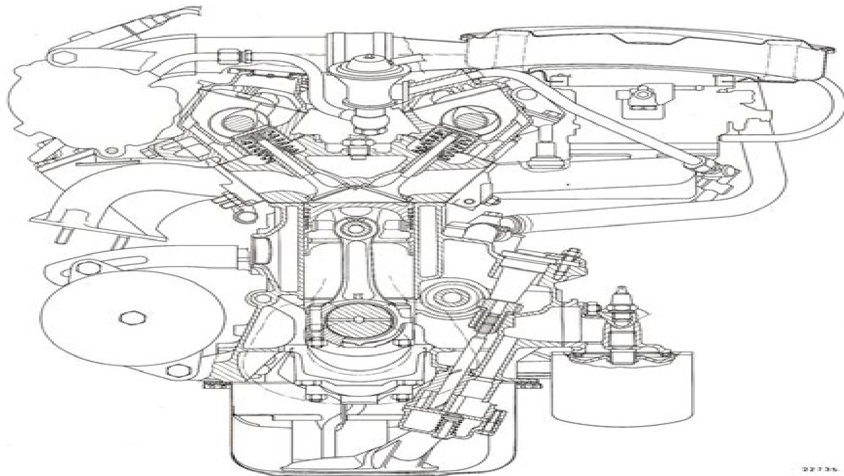
Engine cross section across cylinder (engine 132 A 1.640.4).
