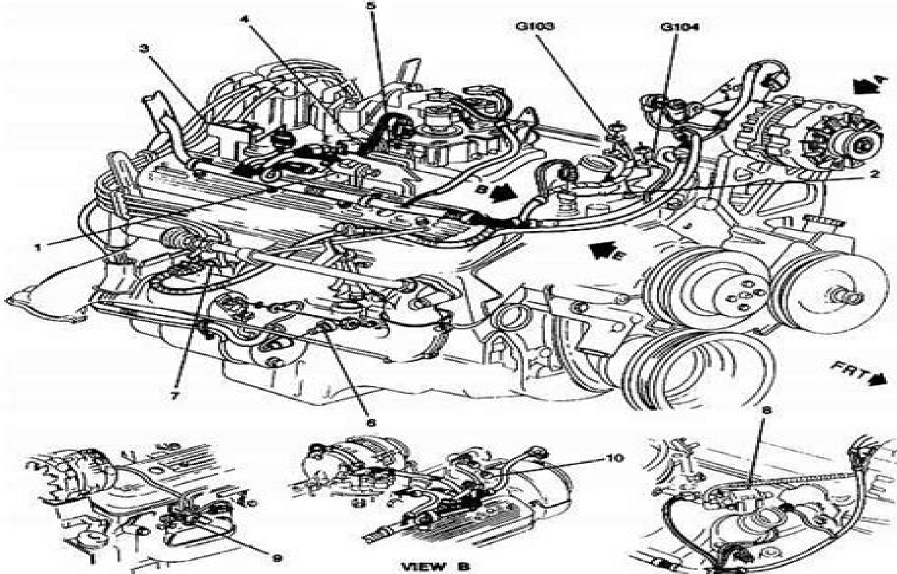
VIEW A
