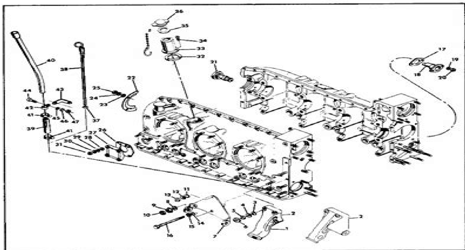
Figure 3. Crankcase Associated Parts.
