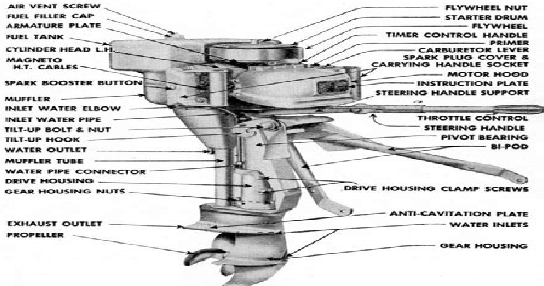
Figure 33. General nomenclature, storm-boat motor.
