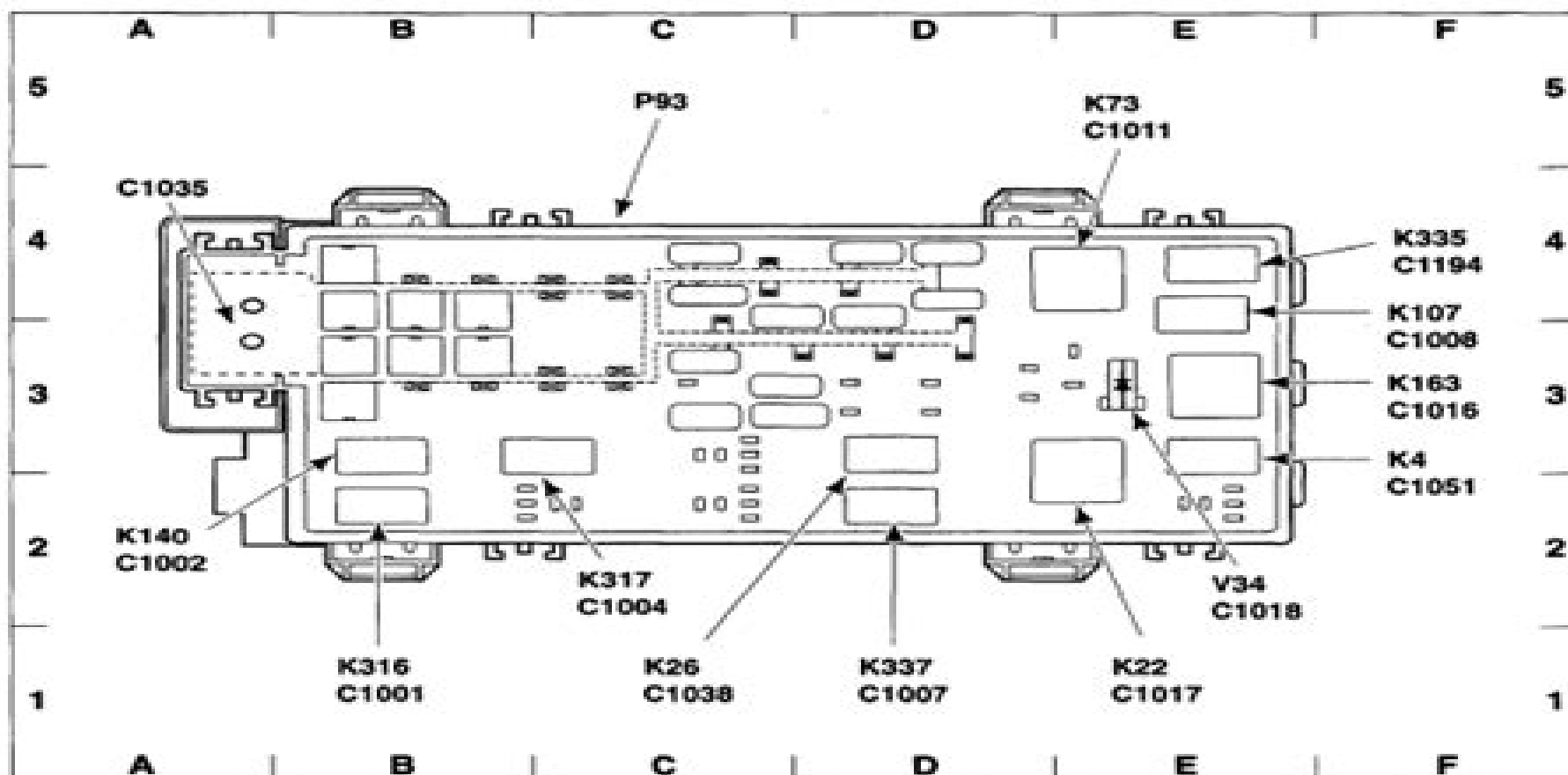
Battery Junction Box (BJB) – 2.5L, 3.0L, 4.0L
