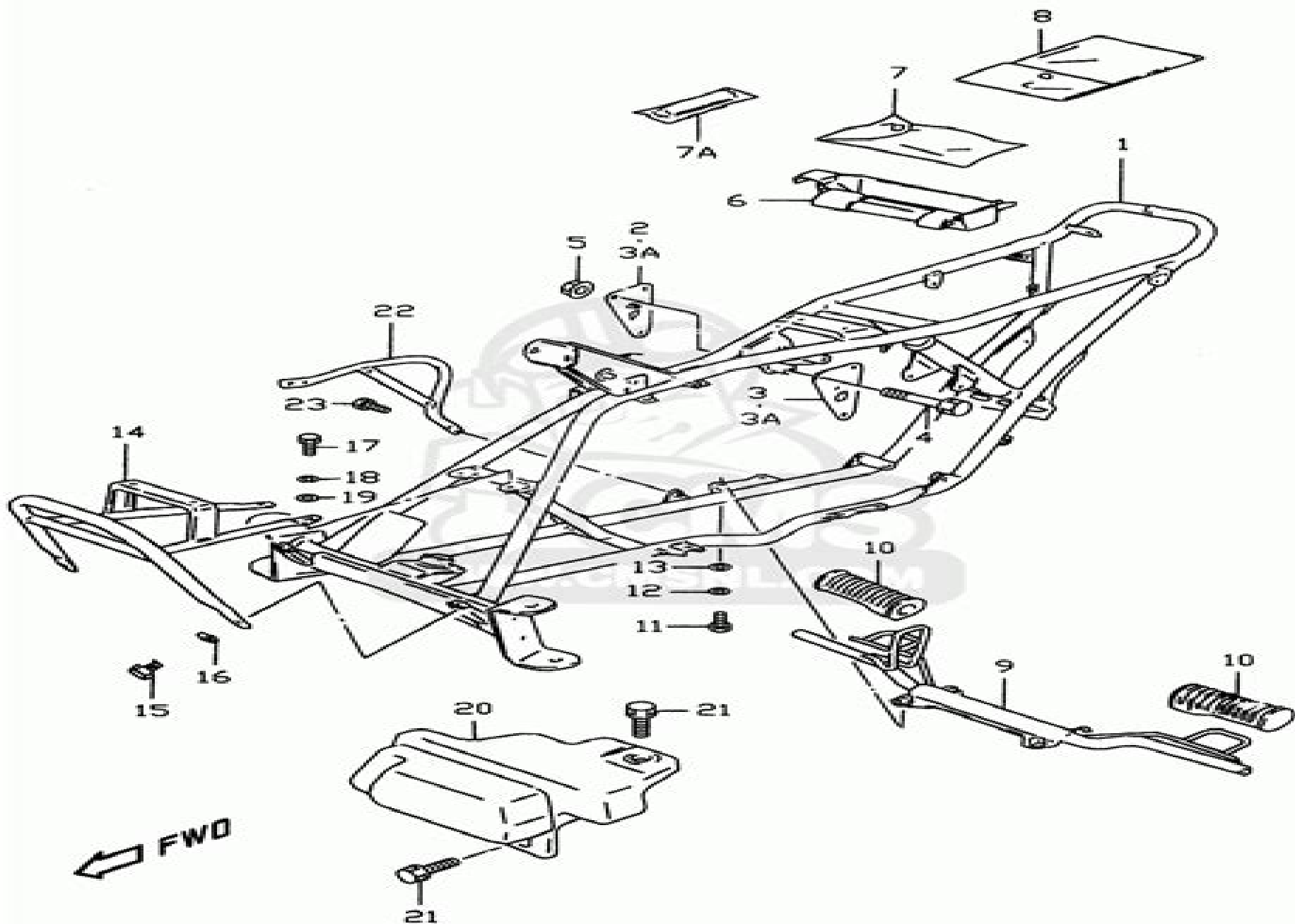
FIG. 14 FRAME - FOOTREST
