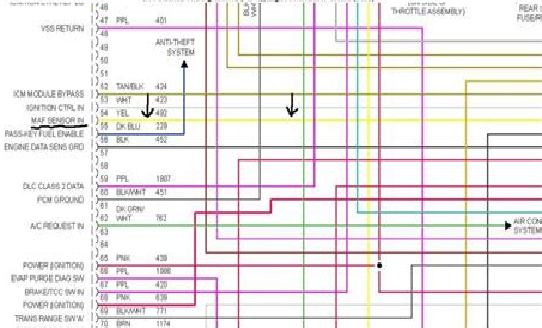
1996 Buick Riviera-Fig. 13: 3.0L (VIN 1), Engine Performance Circuits (1 of 3)
