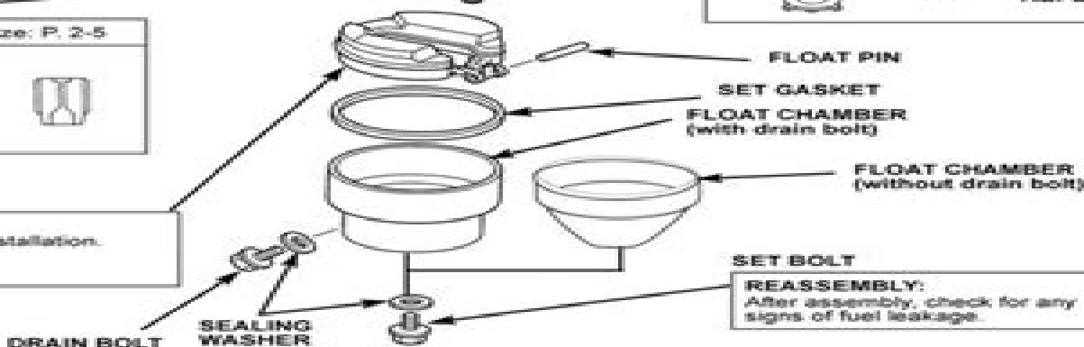
DRAIN BOLT
