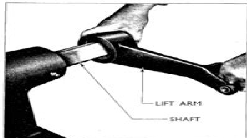
Fig. 195 Fitting a Lift Arm
