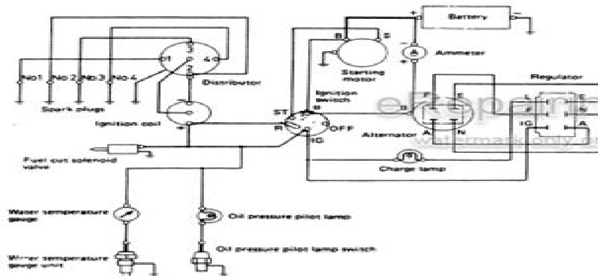
Wiring diagram
