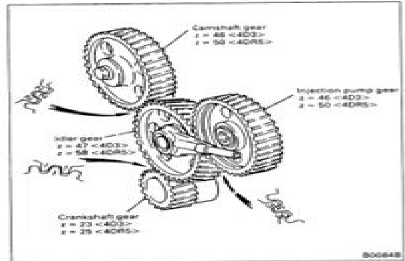
(7) Timing Gear
