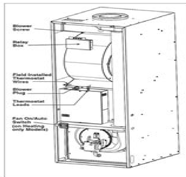
Fig 2. M1* Furnace
