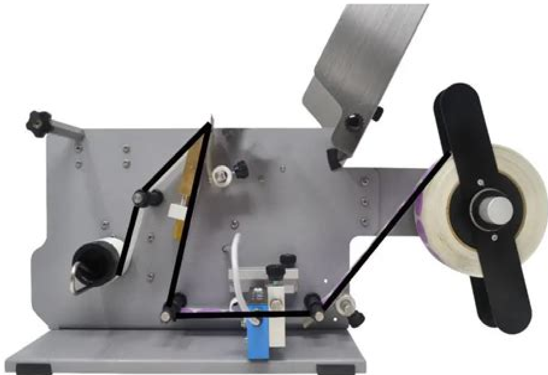
Figure 6 – Label Feeding Diagram Highlighted:
