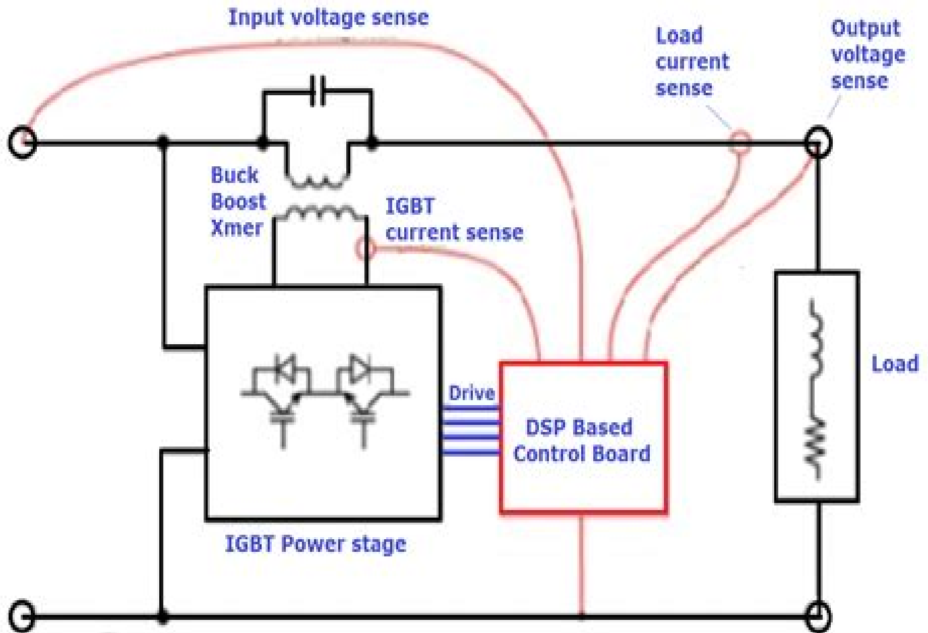
Fig: Block Diagram of Static Voltage Regulator
