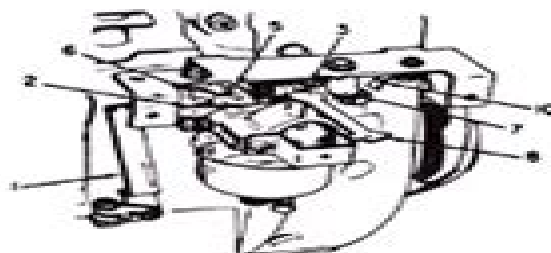
Fig. T35—Mechanical governor linkage. Governed speed of engine is increased by closing loop in linkage (5); decrease speed by spreading loop. Refer to Fig. T33 for legend.
