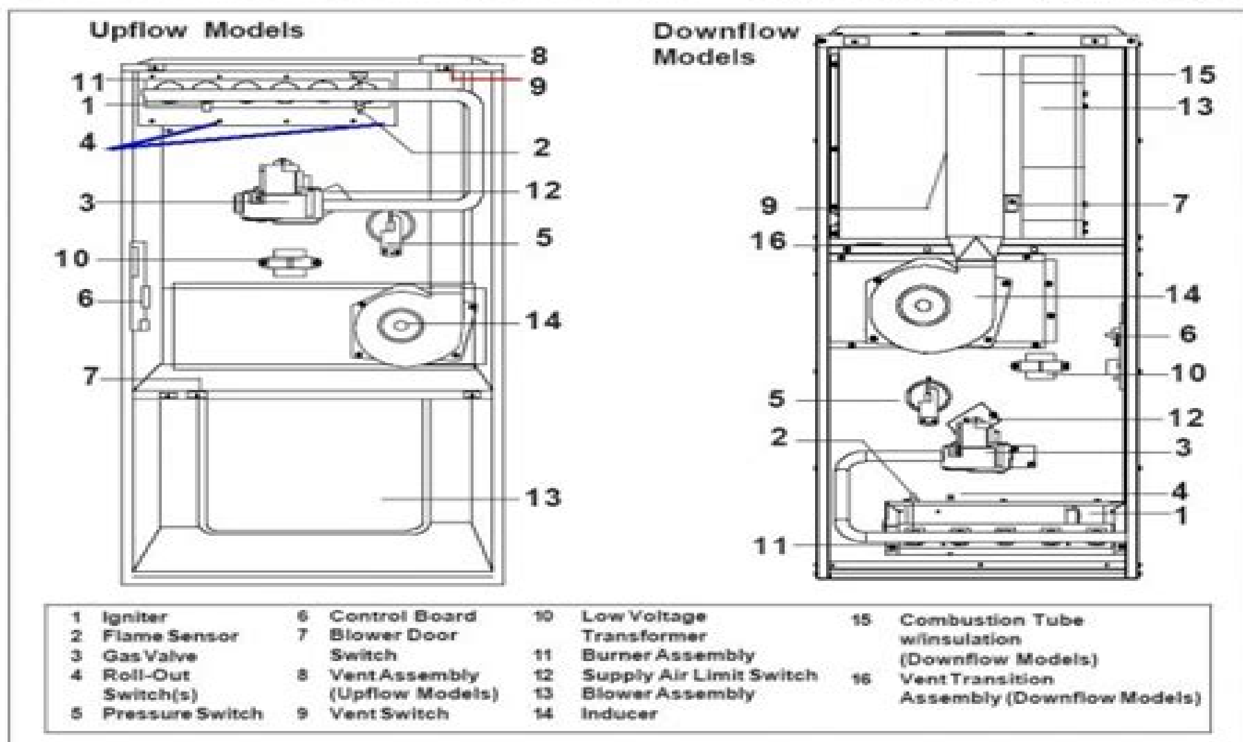
Figure 29. Location of Major Components
