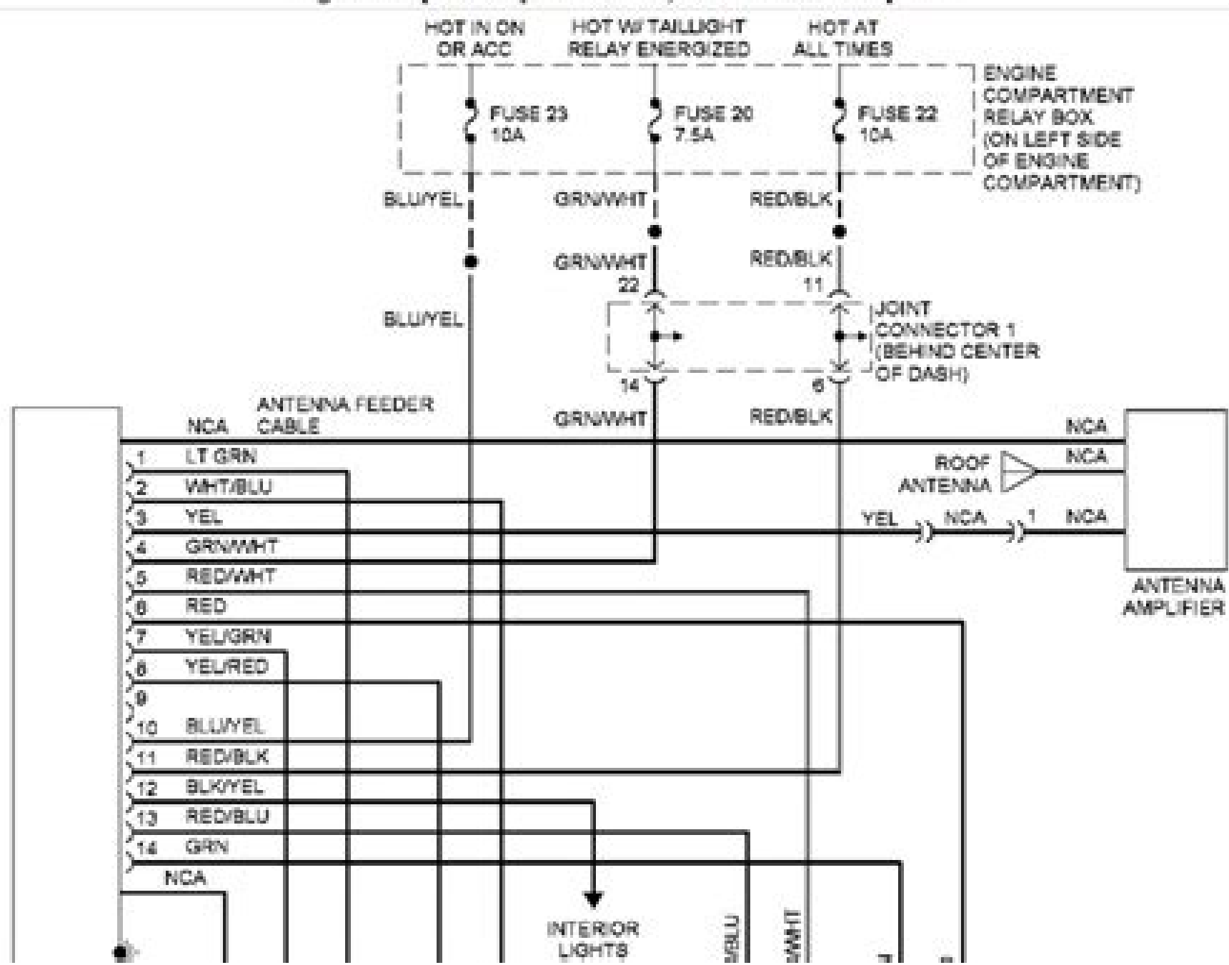
Fig. 68: 6-Speaker System Circuit, Evolution W/O Amplifier
