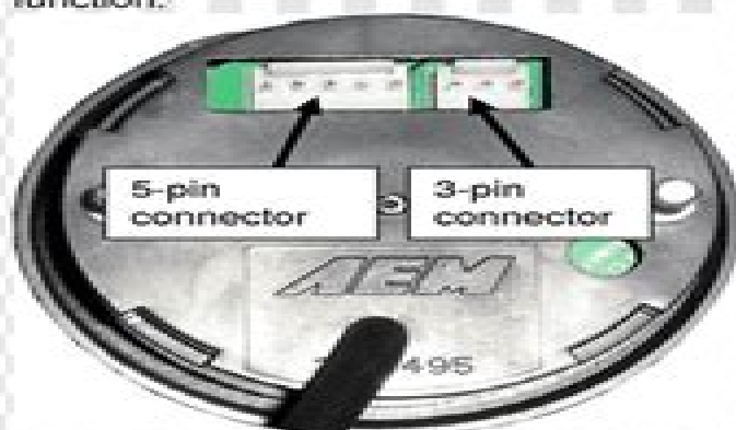
Figure 2. Connector Locations
