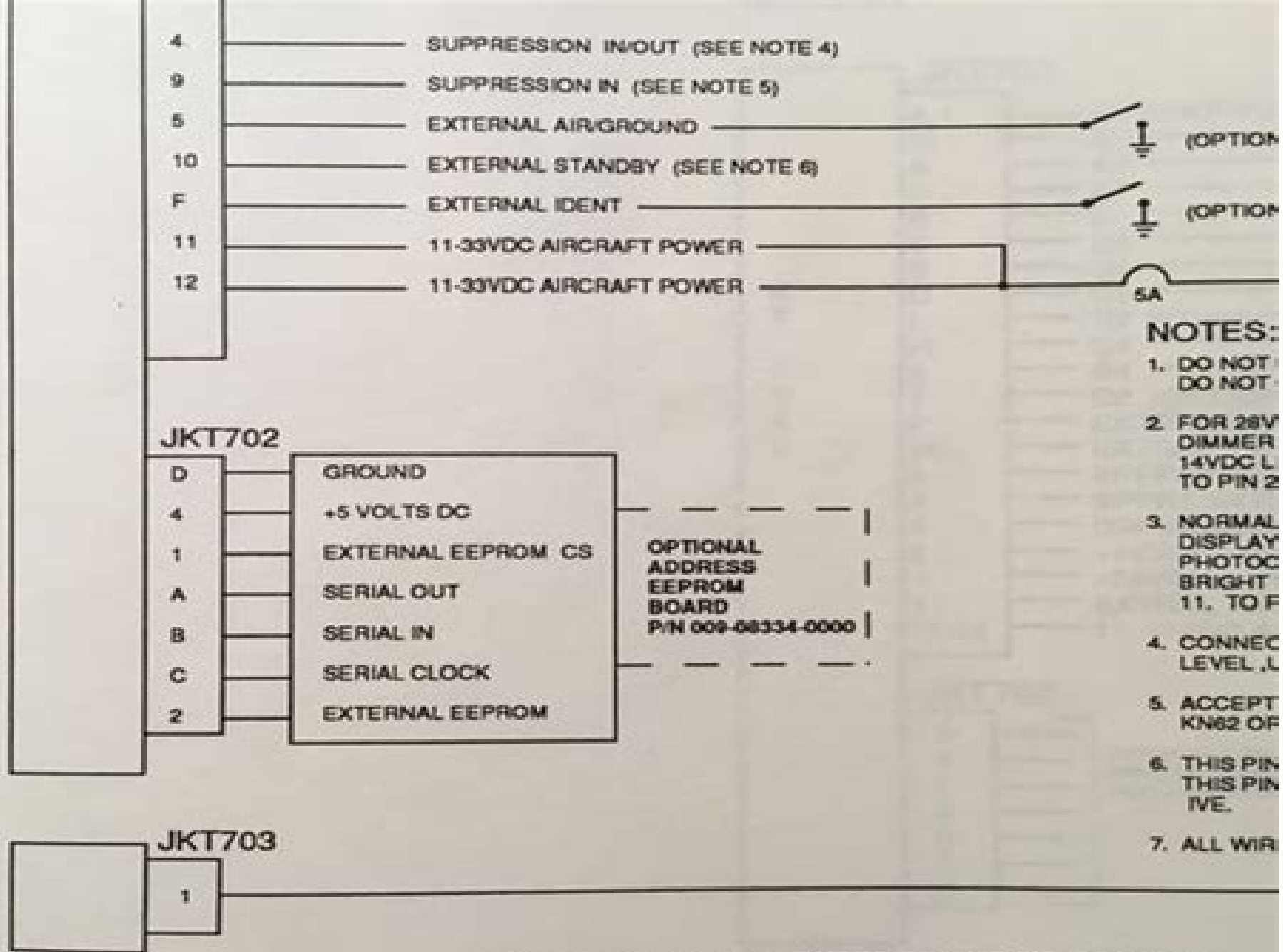
FIGURE 2-1 KT 70 INTERCONNECT DIAGRAM (Sheet 1 of 4)
