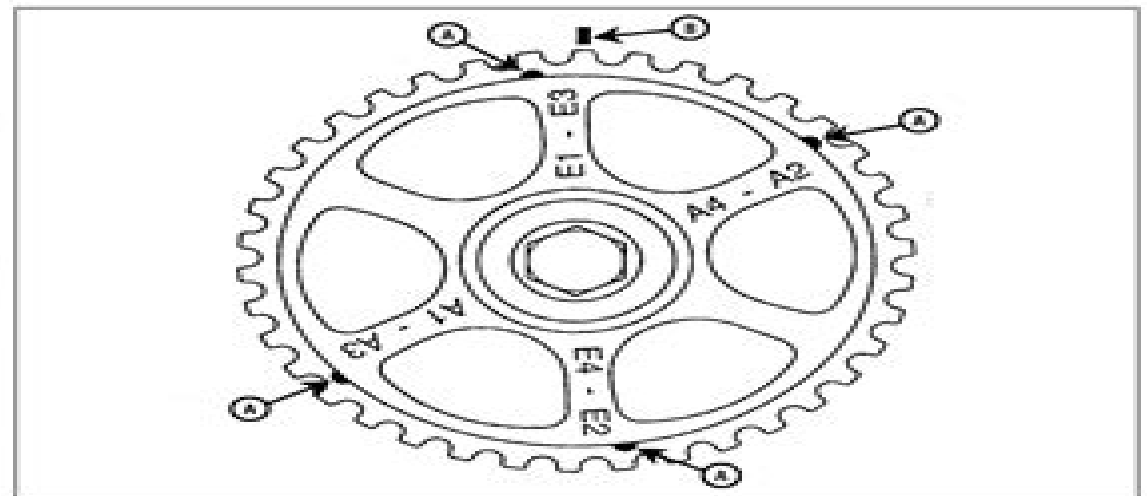
4.6 On the D7F engine, the first of the valve clearance adjustment marks (A), marked E1-E3 on the camshaft sprocket spoke, should be aligned with the reference mark (B) on the valve cover
