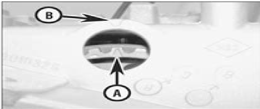
3.6b The TDC timing mark (A) on the camshaft sprocket should align with the reference mark (B) on the top of the lower engine mounting bracket/upper timing belt cover ...
