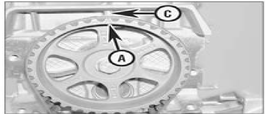
3.6c ... or the reference mark (C) at the top of the valve cover
