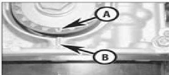
3.7 The timing mark (A) on the crankshaft sprocket should be aligned with the timing mark (B) on the oil pump flange
