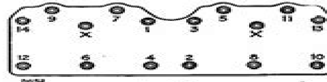
Fig. A-23— Order of tightening cylinder head bolts. Those marked X also secure the rocker shaft.
