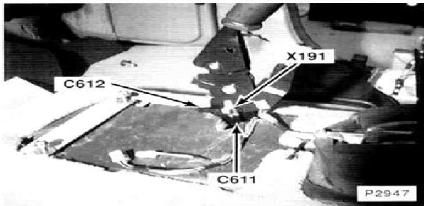
193. beneath centre console on handbrake lever X191 Handbrake Switch C611 (1 – B) C612 (1 – B)
