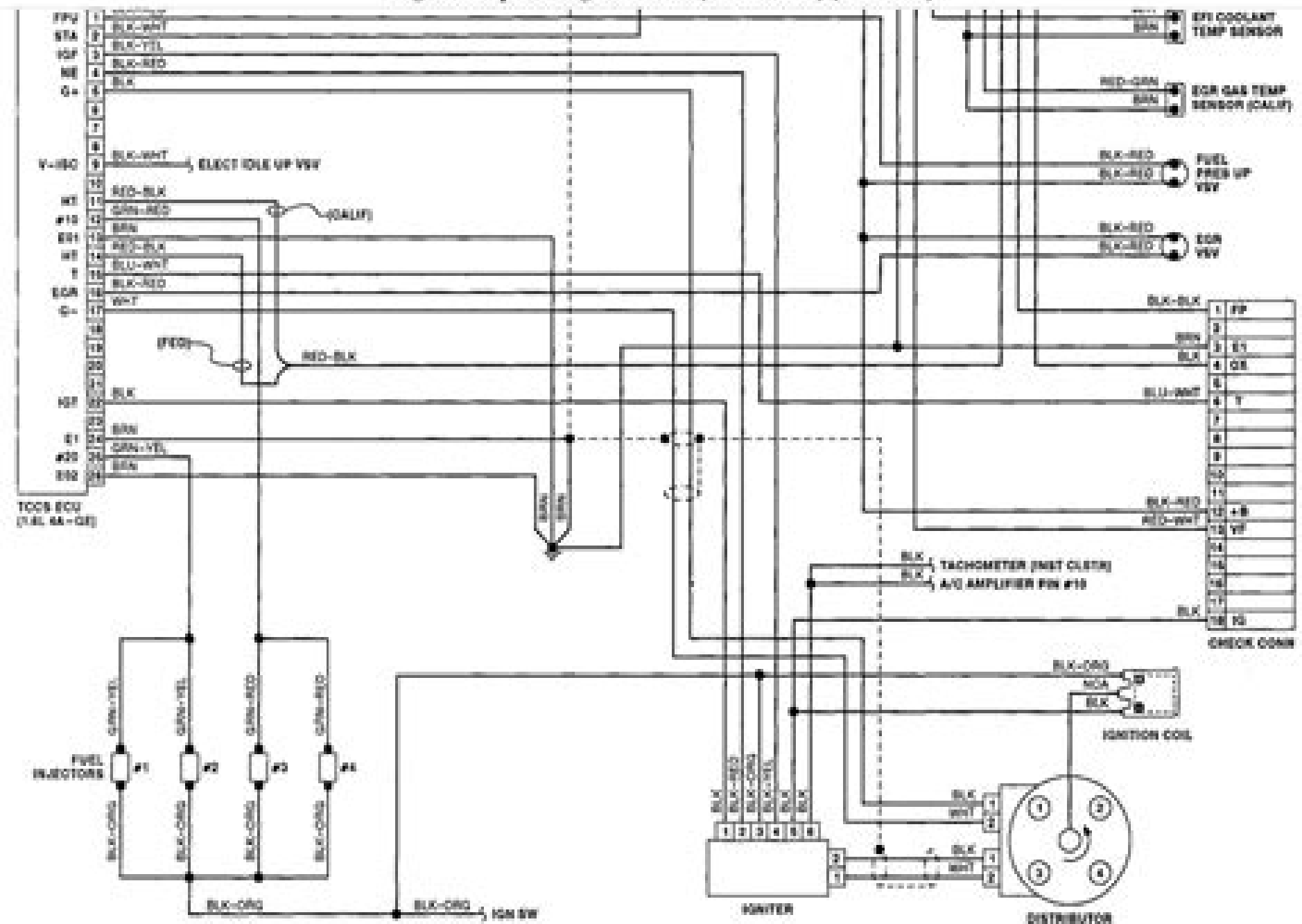
Fig. 3: Computer Engine Control (1.6L 4A-GE) (Grid 8-11)
