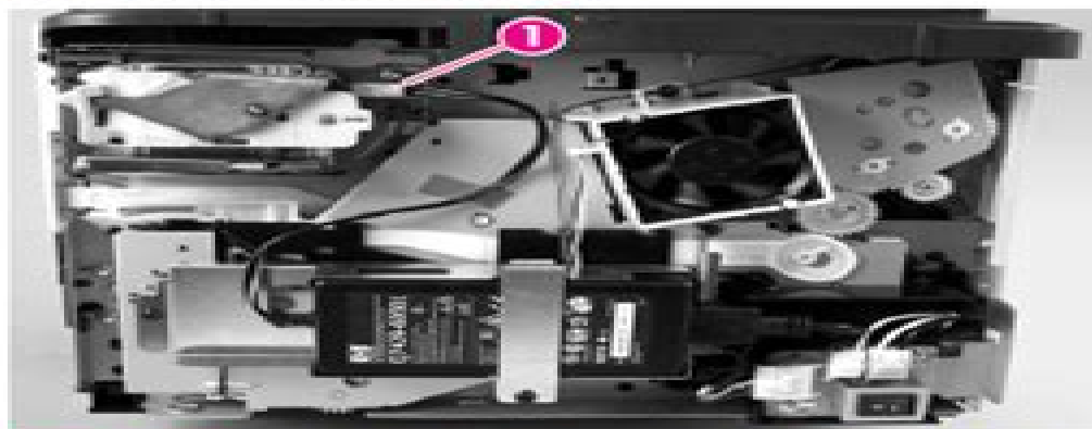
Figure 5-29 Remove the convenience-stapler assembly (1 of 2)
