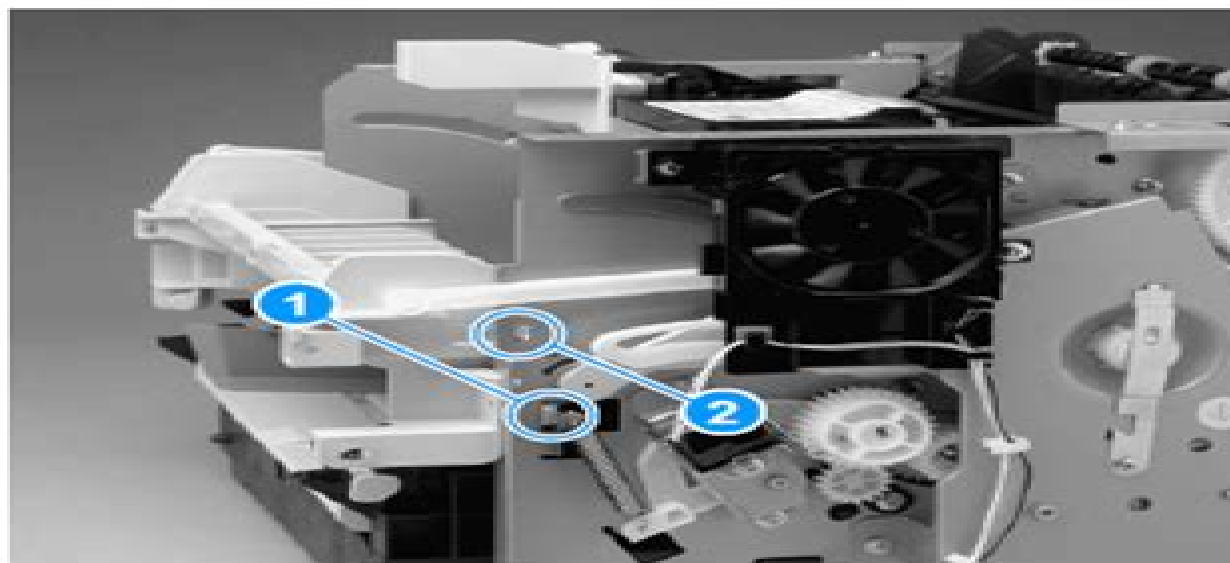
Figure 38. Removing the front guide assembly (2 of 3)
