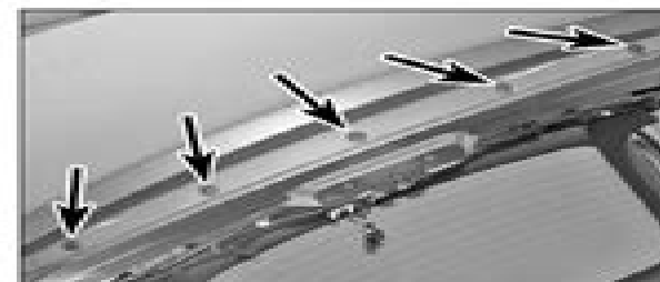
16.14b ... along the lower edge of the tailgate (arrowed)
