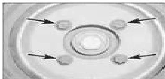
5.4 Crankshaft pulley retaining bolts (removed)
