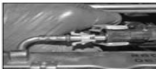
10.15b Releasing the fuel supply pipe quick release with a special tool...
