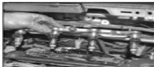
10.16 Remove the fuel rail complete with the injectors
