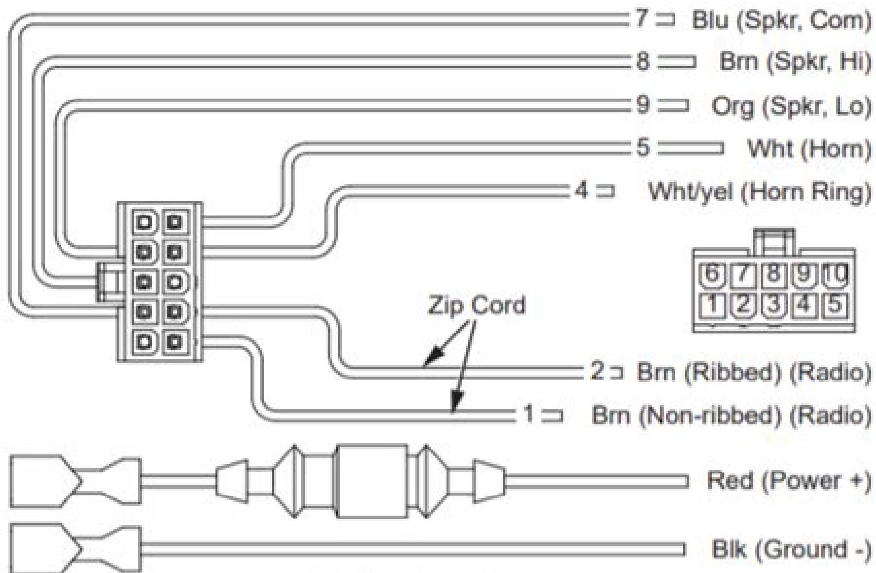
Figure 3 Control Cable Wiring Diagram
