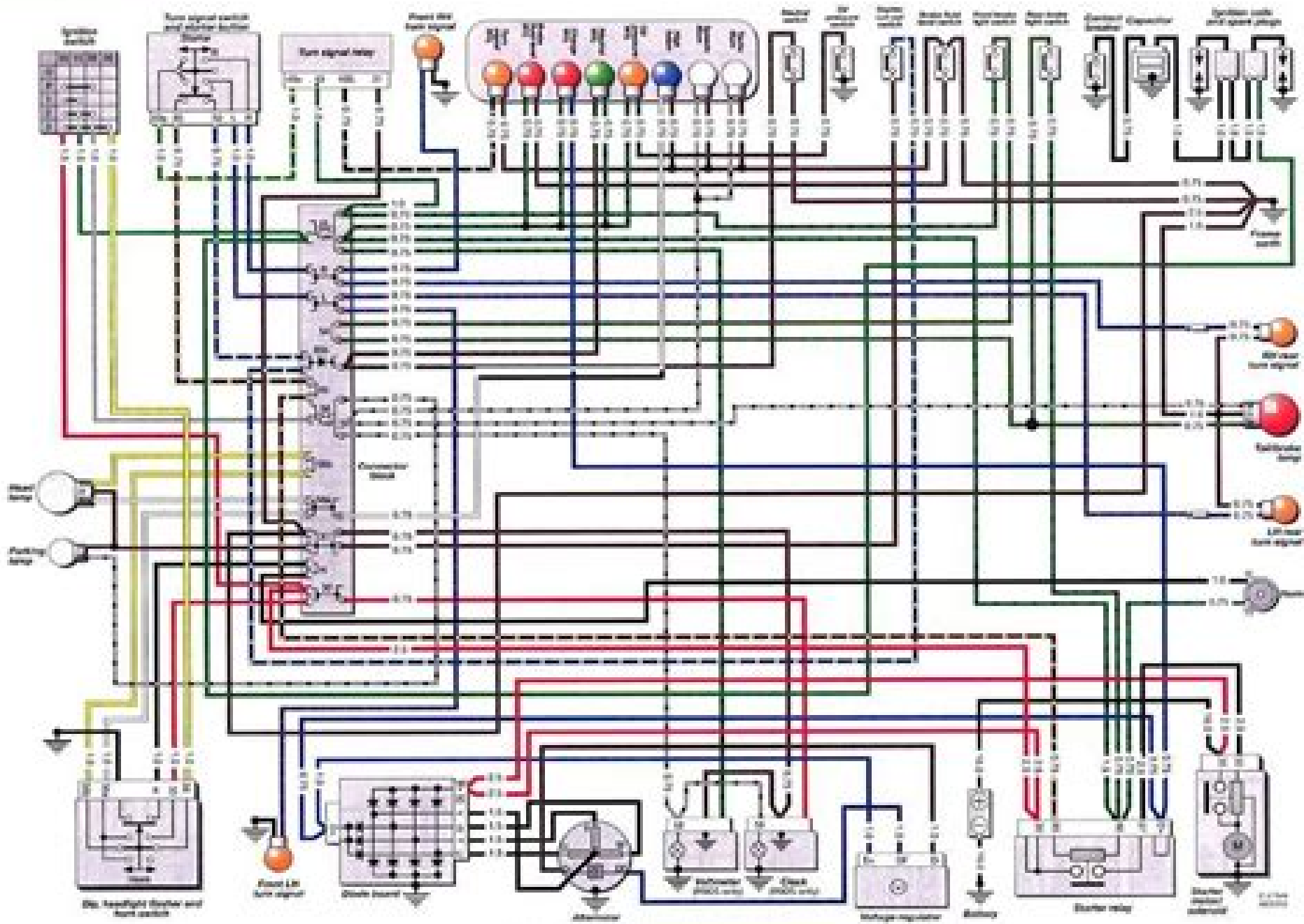
Wiring diagram - 1973 to 1974 /B models
