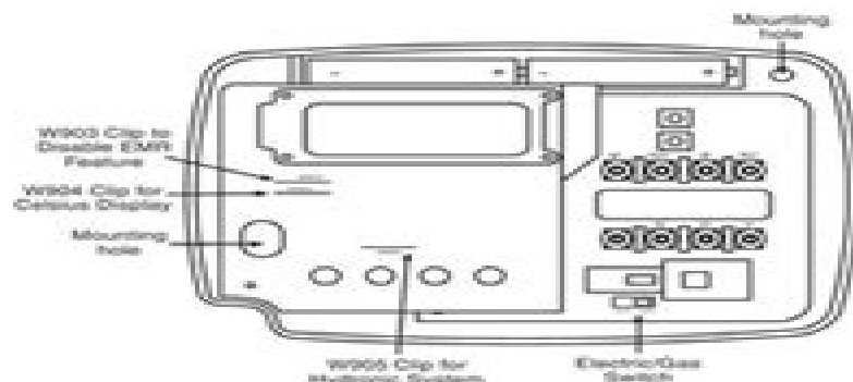
Figure 1. Thermostat base
