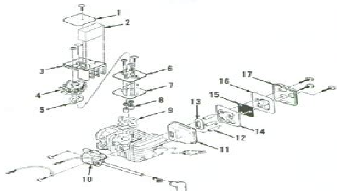
Fig. 10.10—Projected view of intake and exhaust components.
