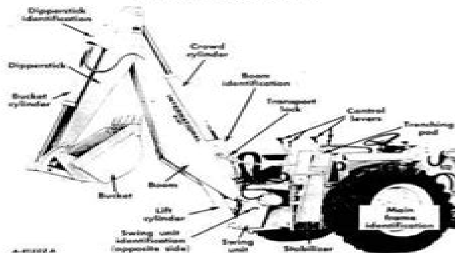
Location of units and parts. International 3121 Backhoe shown on International 2656 Loader Tractor.
