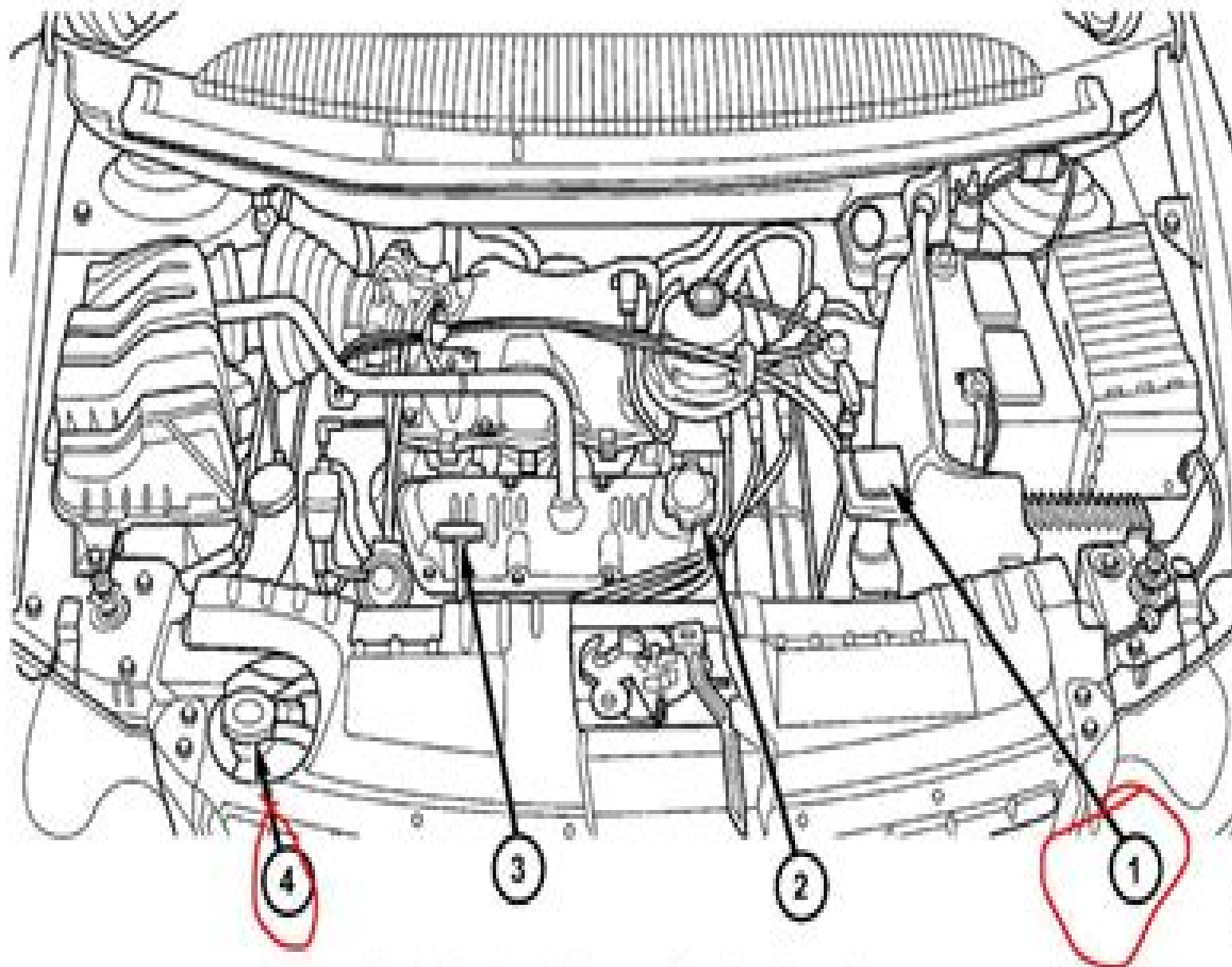
Fig. 6 Cooling System Service Locations
