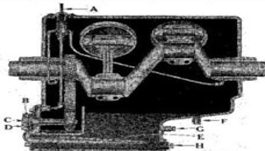
FIG. 18. OILING SYSTEM
